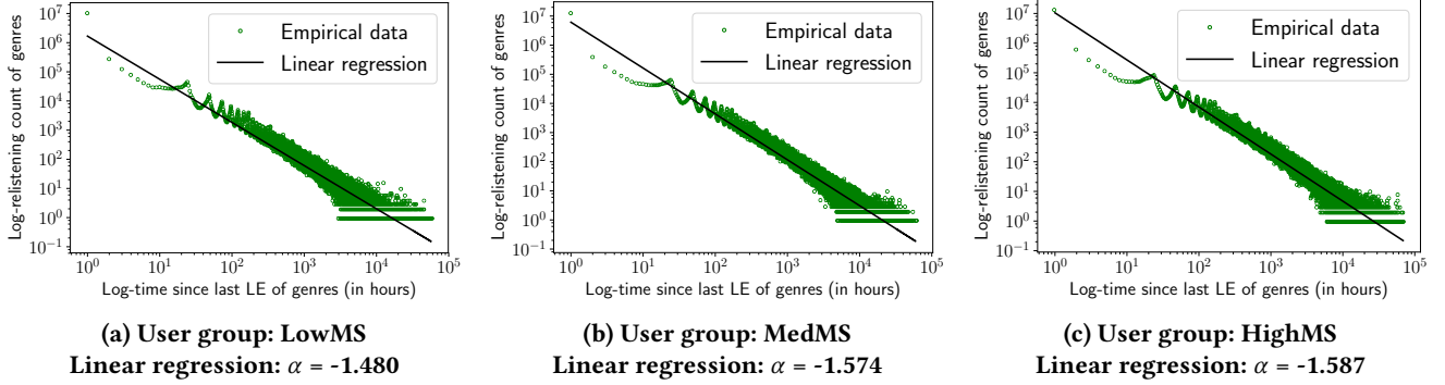
Figure 2: Calculation of the BLL equation’s d parameter. On a log-log scale, we plot the relistening count of the genres over the time since their last LEs. We set d to the slopes \alpha of the corresponding linear regression lines.
